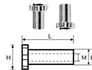
对口螺丝 Butt Screw
