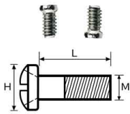
铰链螺丝 Hinge Screw
