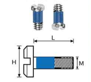
套胶螺丝 Rubber Screw
