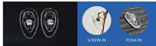
CY033 14.5×8mm CY034 15×8.3mm CY035 15.9×10mm CY036 17×9mm
